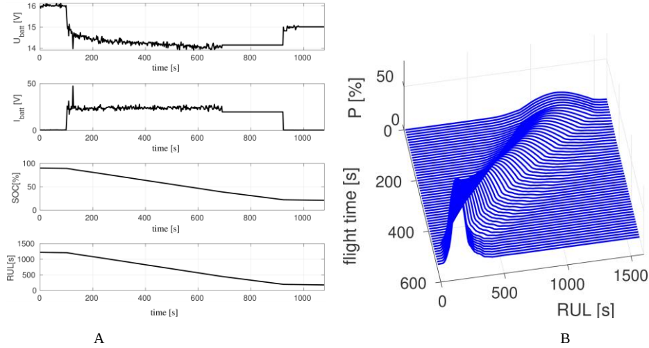
Figure 7: A: Measured battery voltage and current, estimated SOC and RUL for a constant load profile. The UAS takes off at t=100s and touches down at t=700s . The system is turned off at t=930s . B: Probability distribution for RUL over flight time.
