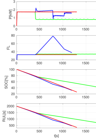
Figure 8: Required power P , altitudes (in flight level (FL)), SOC, and RUL with constant power use for three trajectory variants shown in blue, red and green.
