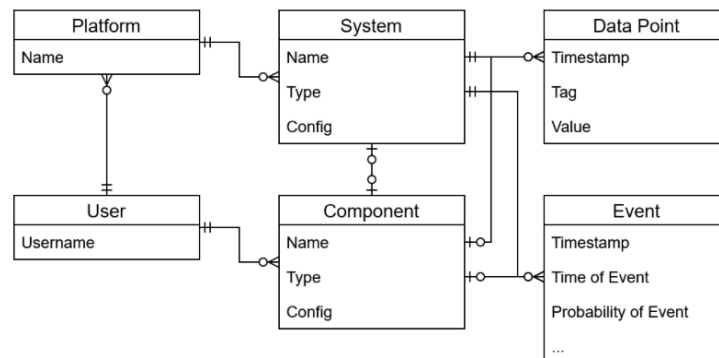
Figure 6: PaaS Entity Relationships
