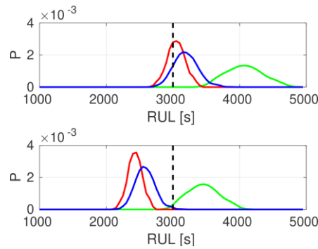
Figure 9: Probability densities for RUL at the beginning of the flight t=0s (top) and at the decision point t=400s (bottom) with \sigma_{pwr} = 0.1 for variants as shown in blue, red, and green.
