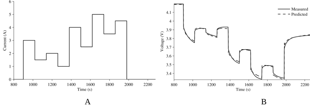
Figure 3: Model validation for variable loading. Current over time (A); measured and predicted discharge curves (B).
