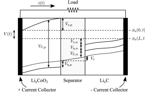
Figure 2: Battery voltages (from [16])
