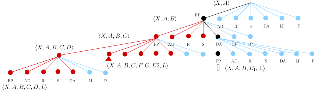
Figure 11: Search tree of DM for situation in Fig. 10. Current path (black), unsuccessfully explored (red), potentially explorable (blue). The small red triangle corresponds to the search along the alternative route [A, B, C, F, G, E_2, L] , which is rejected by prognostics due to insufficient battery resources.
