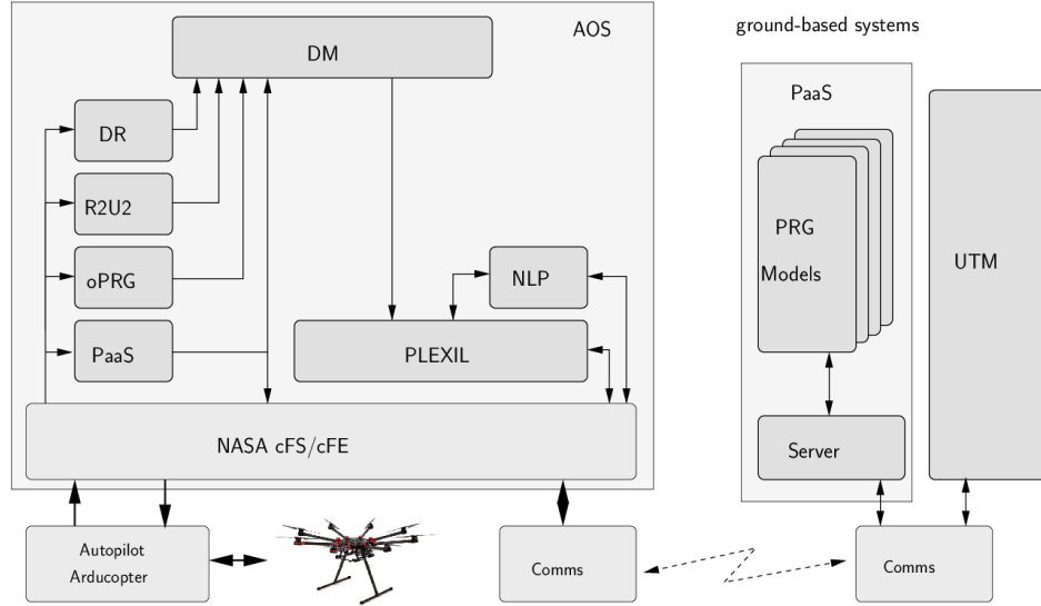
Figure 1: High-level architecture of the AOS system
