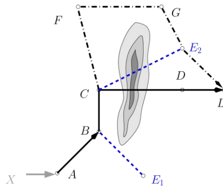
Figure 10: Diagram of waypoints with alternatives (dot-dashed), possible divergence routes (dashed) and emergency airports E 1 , E 2 .
